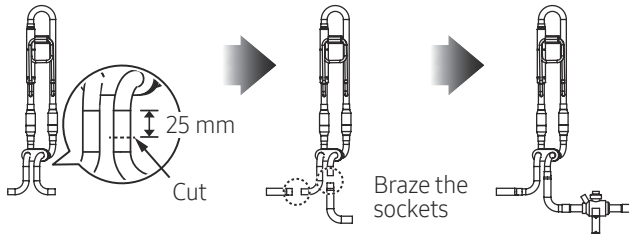
Installation method for AM240H× ~ 260H× (DVM S Large A type)
