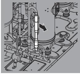
Installation method for AM240H× ~ 260H× (DVM S Large A type)
