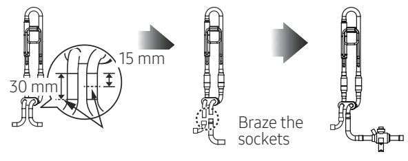
Installation method for AM240K× ~ 300K× (DVM S Large B type)
