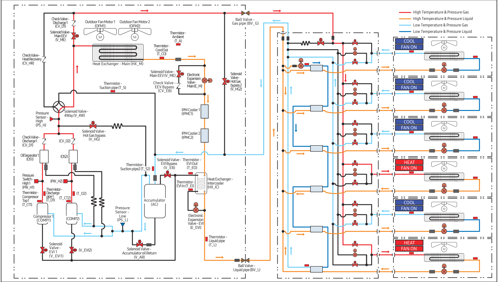
Piping drawings Main Cooling mode
