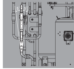
Installation method for AM240K× ~ 300K× (DVM S Large B type)
